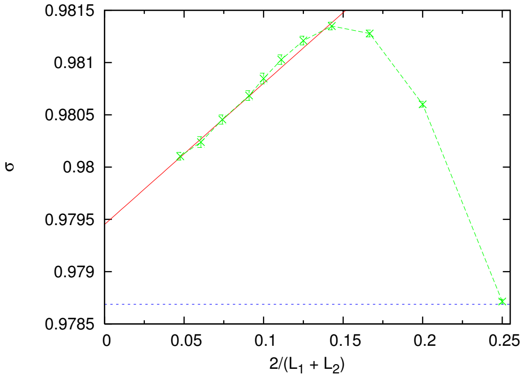
Figure 5: Position \sigma of crossings between d_{L_1}(\sigma) and d_{L_2}(\sigma) on the Nishimori line of the Gaussian random-bond Ising model. The figure also contains a linear fit to the large size data and the value \sigma = 1/1.02177 predicted by duality arguments [21].
