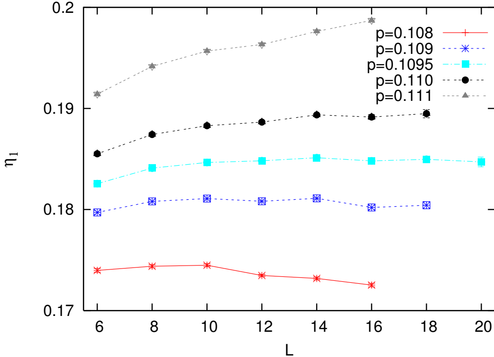
Figure 13: Effective magnetic exponent \eta_1 for p = 0.108, \dots, 0.111 , for the \pm J disorder on the Nishimori line.
