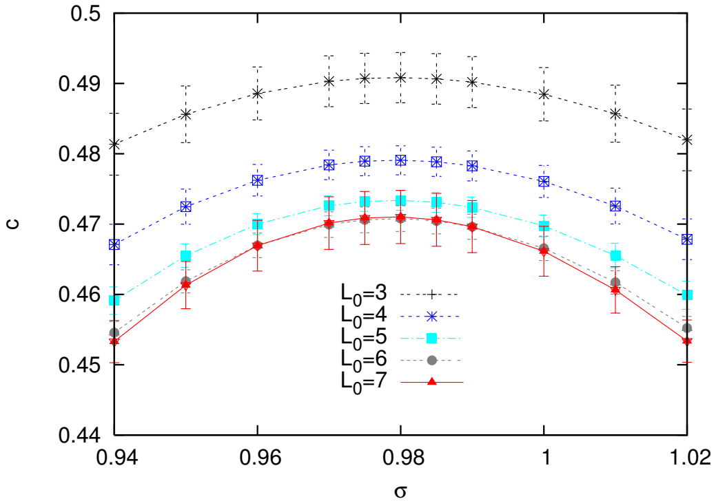
Figure 10: Central charge vs. \sigma along the Nishimori line for the Gaussian distribution of disorder close to the maximum \sigma_c \simeq 0.98 and with L_{\max} = 10 .
