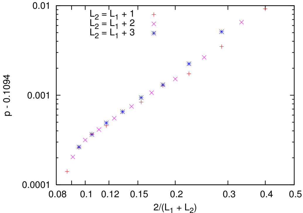
Figure 3: Position p of crossings between d_{L_1}(p) and d_{L_2}(p) on the Nishimori line of the \pm J random-bond Ising model with L_2 \leq 12 .
