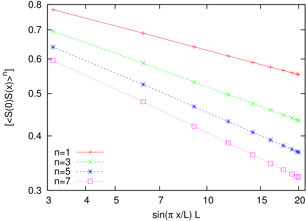
Figure 14: Moments of the spin-spin correlation function for the \pm J RBIM with p = 0.1095 and L = 20 . We only show the odd moments. Error bars are much smaller than the size of the symbols.
