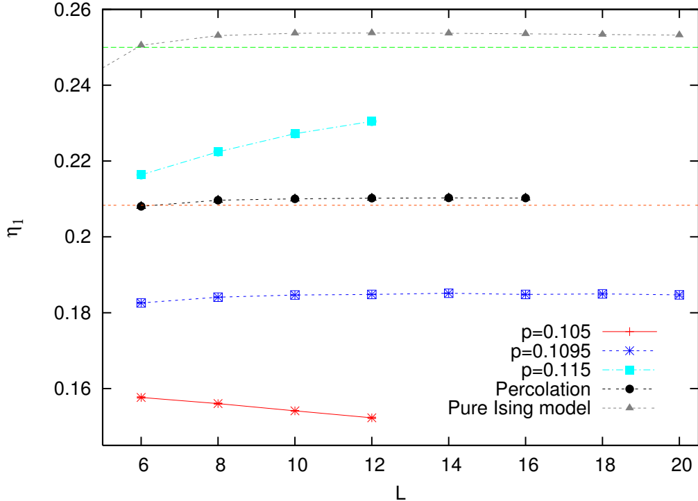
Figure 12: Effective magnetic exponent \eta_1 for the \pm J RBIM with p = 0.105 , p = 0.1095 , p = 0.115 , the percolation model and the pure Ising model.
