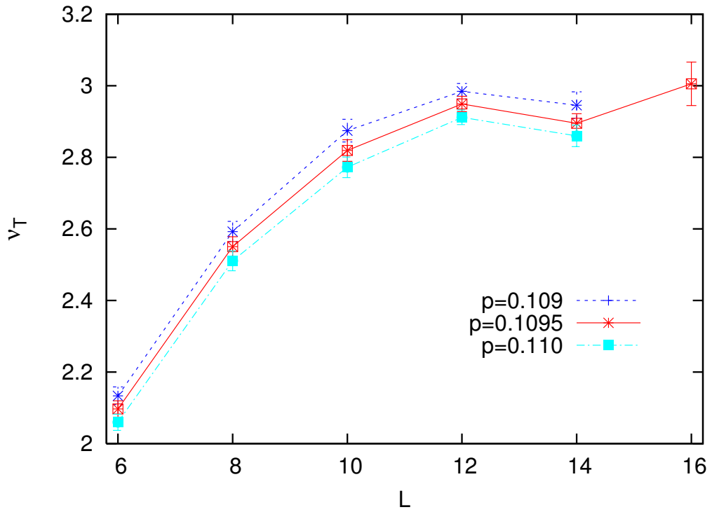
Figure 17: Thermal exponent \nu_T vs. L for the \pm J distribution of disorder.
