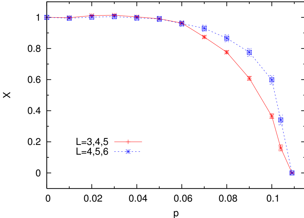
Figure 25: Variation of the effective central charge as characterized by the quantity X (see (8.1)) on the Ferro-Para line, for the J = \pm 1 disorder case.
