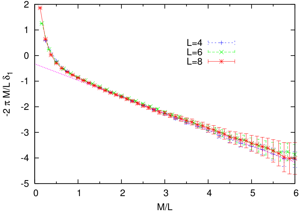
Figure 18: Fit of the free energy for the \pm J RBIM with p = 0.1094 to the form (5.14) in the range 1.5 \leq M/L \leq 5 for L = 4, 6 and 8 .
