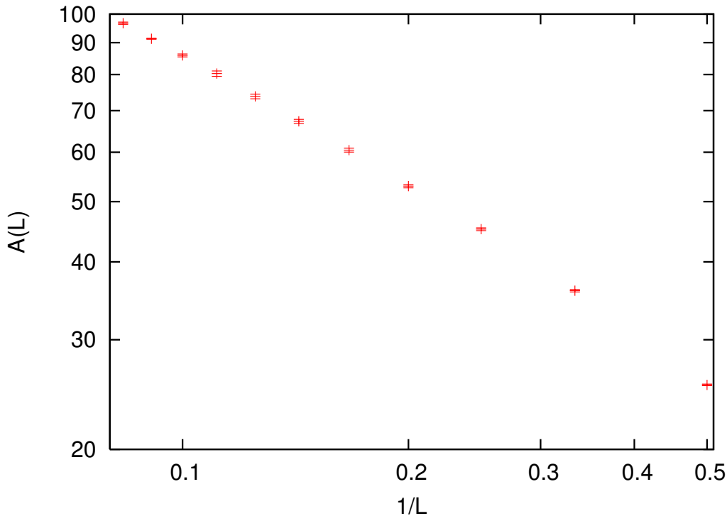
Figure 4: Slope A(L) of the domain-wall free energy for the \pm J random-bond Ising model as a function of 1/L .
