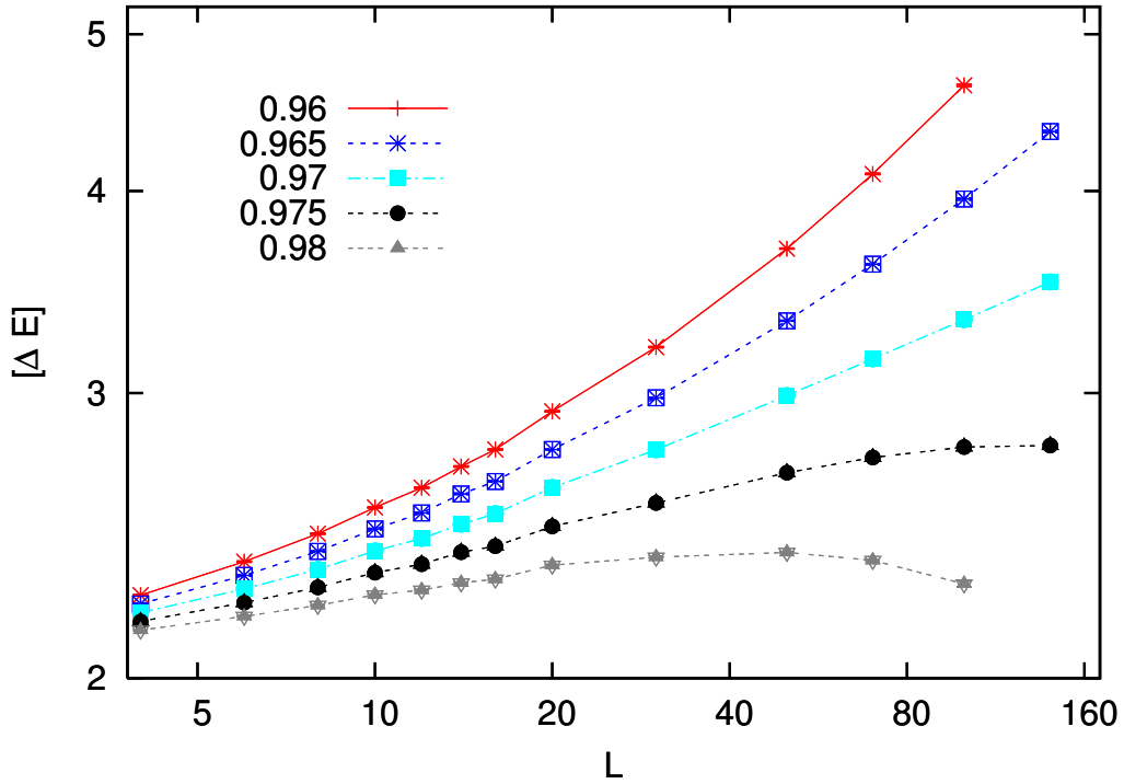
Figure 27: Domain-wall energy [\Delta E] as a function of the system size L for the Gaussian disorder at T = 0 and for \sigma = 0.96, \dots, 0.98 .
