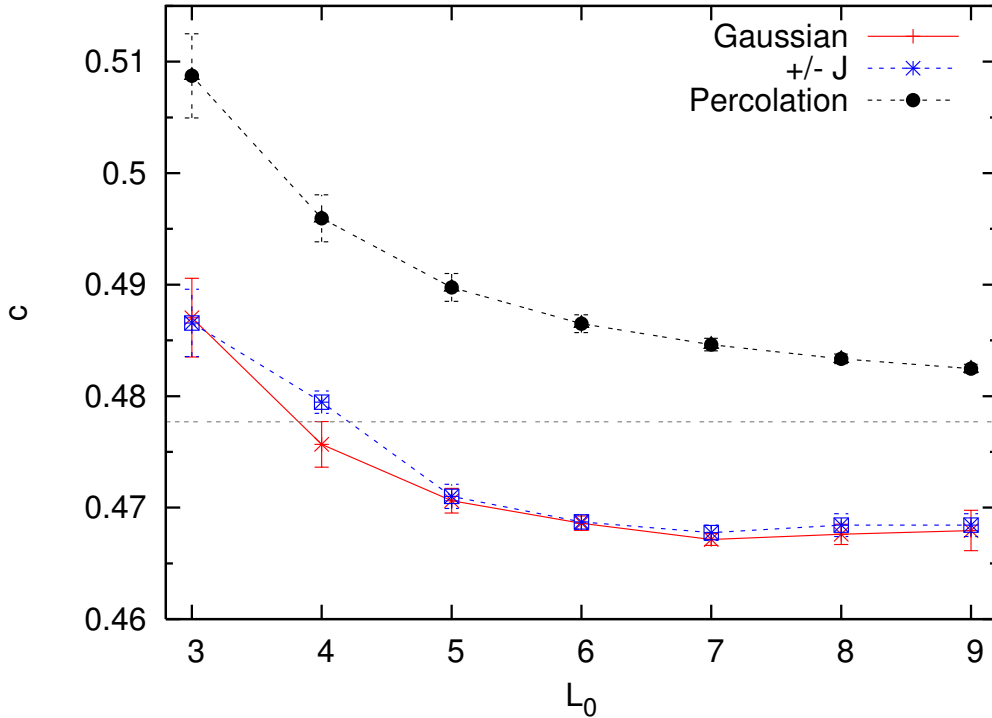
Figure 11: Central charge at the multicritical fixed point on the Nishimori line for the \pm J and Gaussian distributions of disorder. We also show for comparison finite-size estimates of the central charge for percolation. The horizontal line shows the infinite system limit c = \frac{5\sqrt{3}\ln 2}{4\pi} for percolation on Ising clusters [41].
