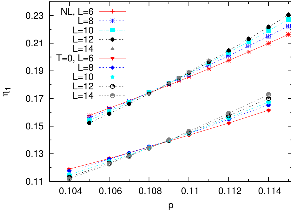
Figure 29: Effective magnetic exponent \eta_1 vs. p for \pm J disorder case on the Nishimori line and at T = 0 .
