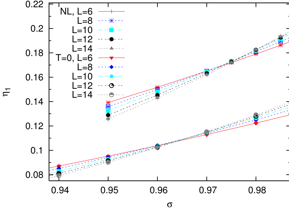
Figure 30: Effective magnetic exponent \eta_1 vs. \sigma for Gaussian disorder on the Nishimori line and at T = 0 .
