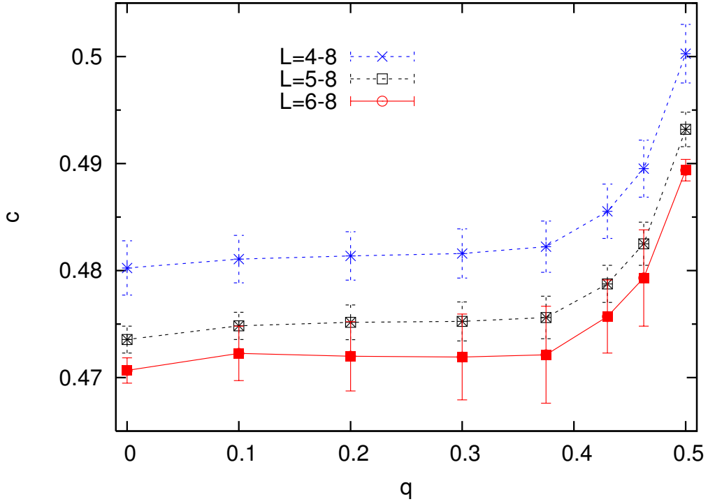
Figure 21: Central charge vs. dilution q along the intersection of the p - q - T Nishimori surface with the paramagnetic-ferromagnetic critical surface for the \pm J disorder case.
