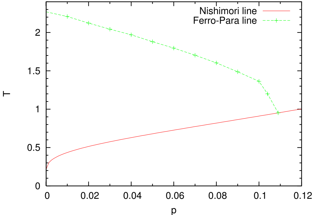
Figure 24: T - p phase diagram for the J = \pm 1 disorder case.
