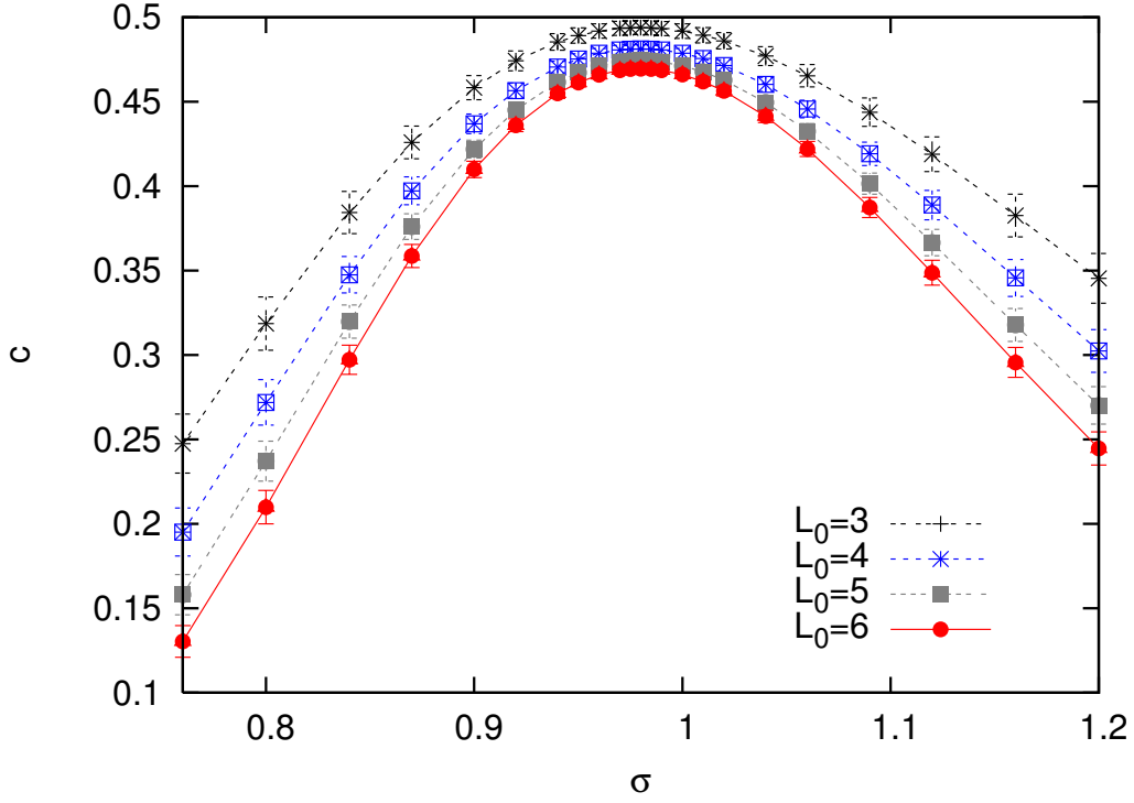
Figure 9: Central charge vs. \sigma along the Nishimori line for the Gaussian distribution of disorder, with L_{\max} = 8 .
