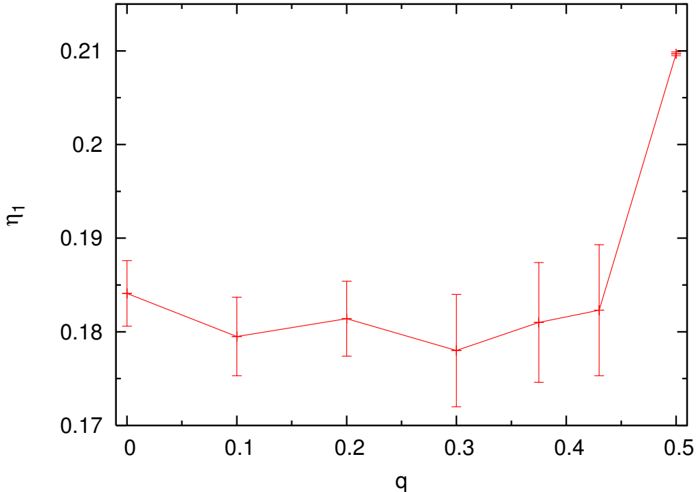
Figure 23: Magnetic exponent \eta vs. dilution q along the intersection of the p - q - T Nishimori surface with the paramagnetic-ferromagnetic critical surface for the \pm J disorder case.
