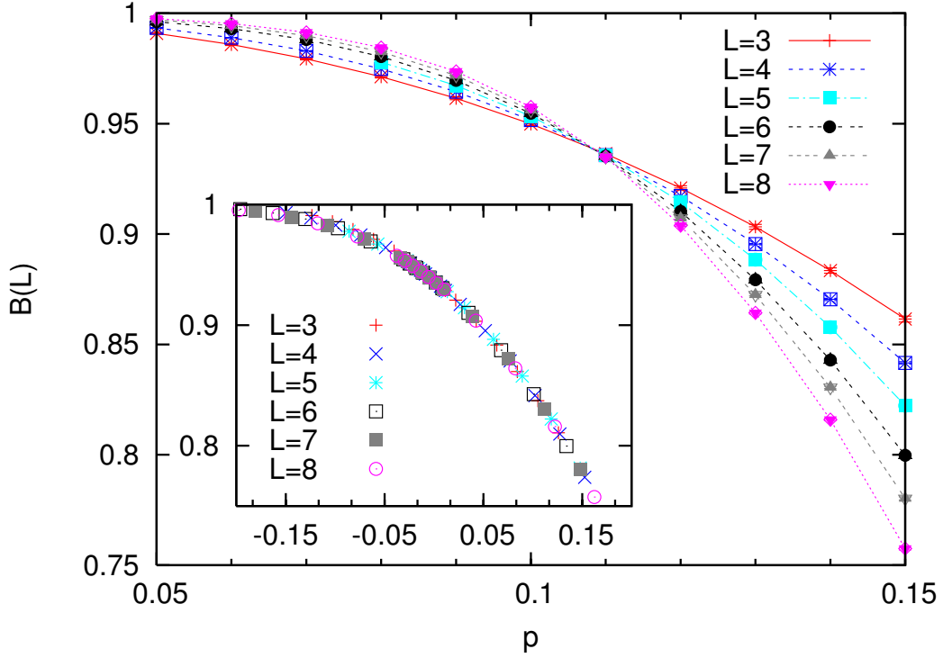
Figure 19: B(L) vs. p on the Nishimori line for the \pm J disorder case. The inset shows B(L) vs. (p - p_c)L^{1/\nu} , with p_c = 0.1094 and \nu = 3/2 .
