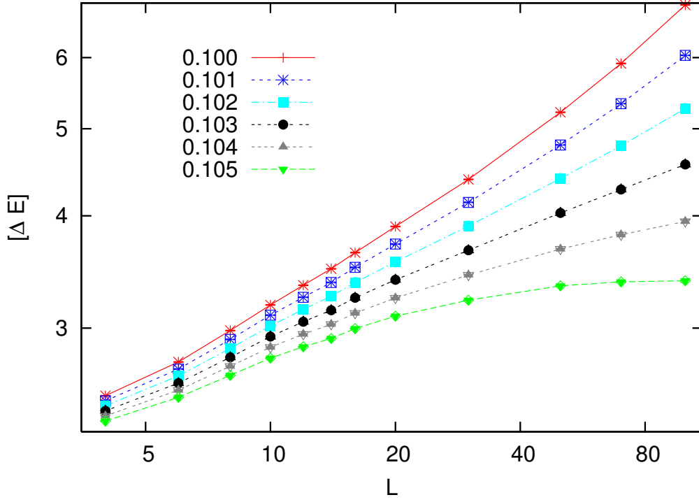
Figure 26: Domain-wall energy [\Delta E] as a function of the system size L for the \pm J disorder at T = 0 and for p = 0.100, \dots, 0.105 .
