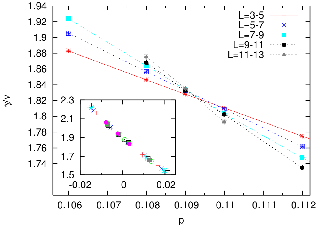
Figure 20: Susceptibility exponent \gamma/\nu vs. p on the Nishimori line for the \pm J disorder case. The inset shows \chi(L)L^{-\gamma/\nu} vs. (p - p_c)L^{1/\nu} , with p_c = 0.1094 and \nu = 3/2 .
