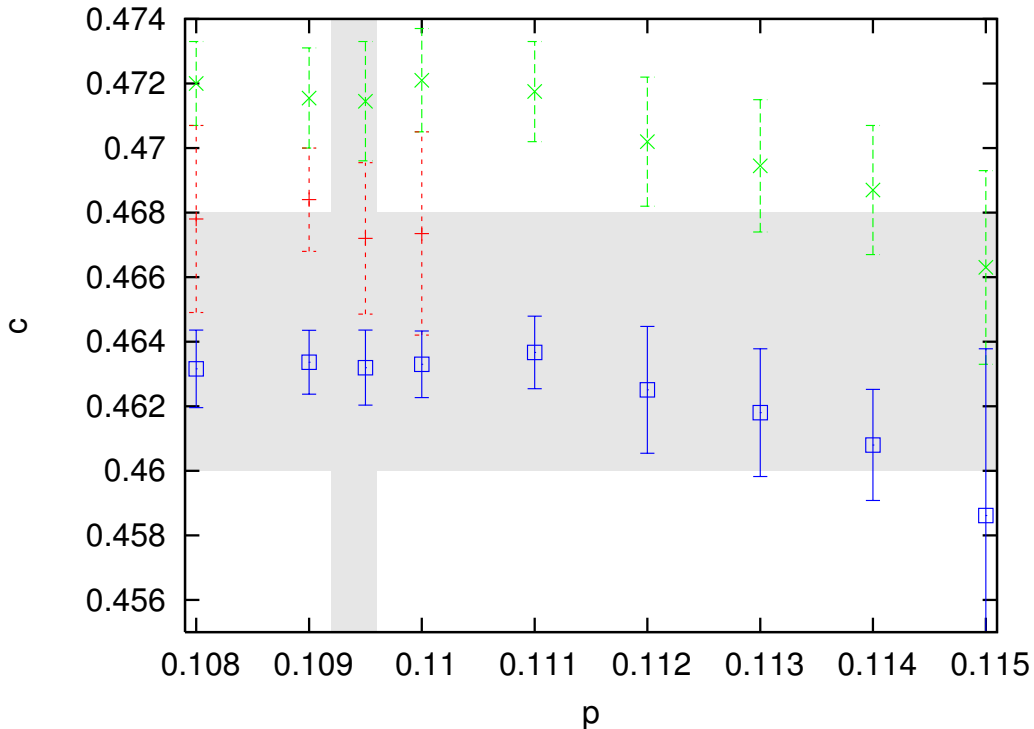
Figure 8: Estimates for the central charge c along the \pm J Nishimori line (2.4) in the vicinity of the Nishimori point obtained from (4.1) for 5 \leq L \leq 9 (' \times '), 6 \leq L \leq 12 ('+') or (4.2) with 4 \leq L_0 \leq 6 (boxes). The grey shaded areas denote our final confidence intervals for p_c (vertical) and the central charge (horizontal).
