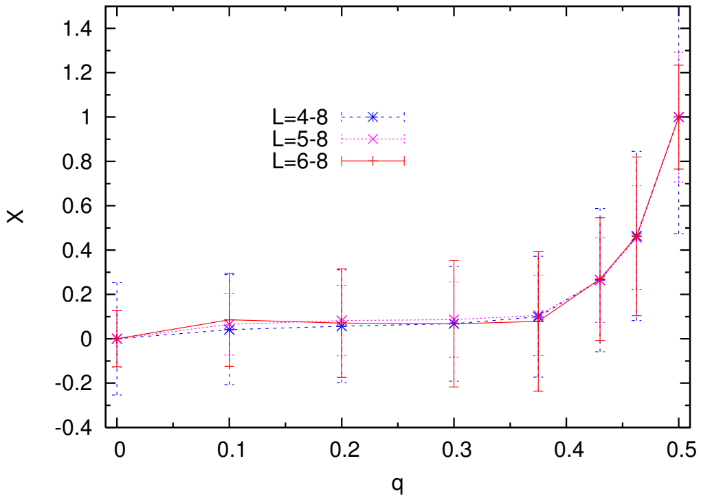
Figure 22: X vs. dilution q along the intersection of the p - q - T Nishimori surface with the paramagnetic-ferromagnetic critical surface for the \pm J disorder case.
