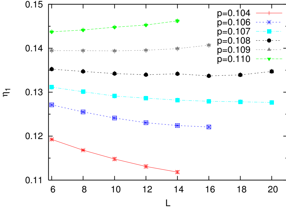
Figure 28: Effective magnetic exponent \eta_1 vs. L for the \pm J disorder case at T = 0 .
