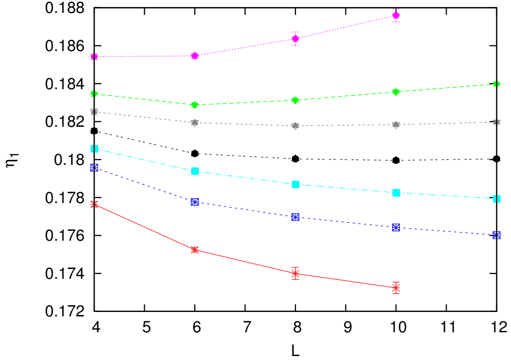
Figure 16: Effective magnetic exponent \eta_1 vs. L for the Gaussian distribution of disorder with \sigma = 0.976, 0.978, 0.979, 0.980, 0.981, 0.982, 0.984 (from bottom to top).
