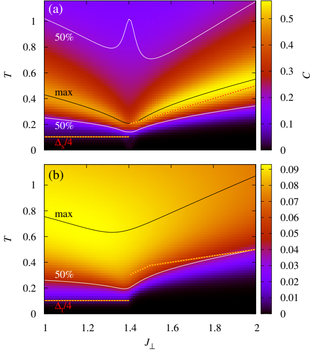
FIG. 10. (Color online) Exact diagonalization results for the specific heat, C (a), and susceptibility, \chi (b), of the fully frustrated ladder ( J_x = J_{\parallel} = 1 ) with L = 14 rungs, shown for the full range of J_{\perp}/J_{\parallel} ratios around the transition. Black lines mark the positions, T_{\max}^C and T_{\max}^{\chi} , of the peaks in both quantities. White lines mark the temperatures, T_{\text{half}}^C and T_{\text{half}}^{\chi} , where they have reached half of the peak height, and for C(T) the temperature, T_u^C , where the peak has fallen again to half of the peak height as T continues to increase. Red-yellow dashed lines mark 1/4 of the gaps relevant for each quantity, which for C(T) is the minimum gap \Delta_s and for \chi(T) the triplet gap \Delta_t (Subsec. II A).
