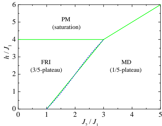
FIG. 4. Ground-state phase diagram of the spin-1/2 Ising-Heisenberg model on a diamond-decorated square lattice in the J_2/J_1 - h/J_1 plane. The notation for the various ground states is as follows: FRI – classical ferrimagnetic phase, MD – quantum monomer-dimer phase and PM – saturated paramagnetic phase. The dashed blue line shows the projection of the critical condition (14) onto the J_2/J_1 - h/J_1 plane.
