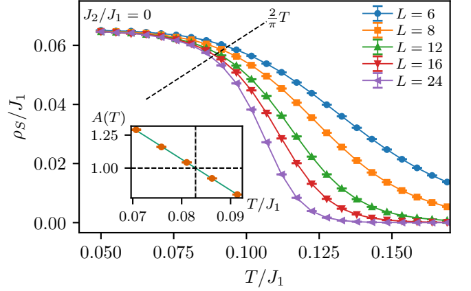
FIG. 17. Spin stiffness \rho_S for different system sizes L as a function of temperature T/J_1 for the diamond-decorated square lattice model at J_2/J_1 = 0 and h/J_1 = 4.5 . The dashed line denotes the scaling form of the universal jump. The inset shows the quantity A(T) from the finite-size scaling analysis. The KT transition temperature is denoted by the dashed vertical line, where A(T) = 1 holds, obtained using a linear fit (solid line).
