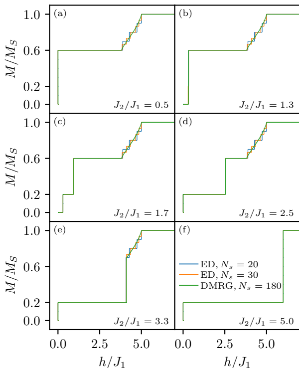
FIG. 5. Zero-temperature magnetization curves of the spin-1/2 Heisenberg antiferromagnet on a diamond-decorated square lattice as obtained from full exact diagonalization and DMRG method for system sizes N_s = 20 , N_s = 30 and N_s = 180 , respectively, for several values of the interaction ratio J_2/J_1 . In all plots, the total magnetization M is scaled with respect to its saturated value M_S .
