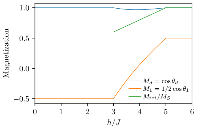
FIG. 16. Local magnetizations M_1 and M_d of the two inequivalent sites of the classical mixed-spin Heisenberg model on the Lieb lattice as well as the total magnetization M_{\text{tot}} (normalized by the saturated magnetization M_S ) as a function of the magnetic field h/J at zero temperature.
