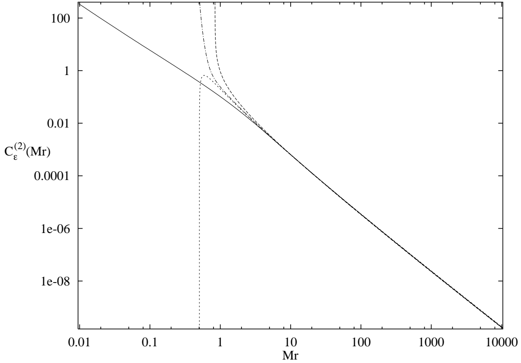
Figure 1: Two-particle approximation to the correlation function of the energy operator (full line), the one-loop perturbative result (long dashes), the two-loop result (short dashes) and the three-loop result (dot-dashes).
