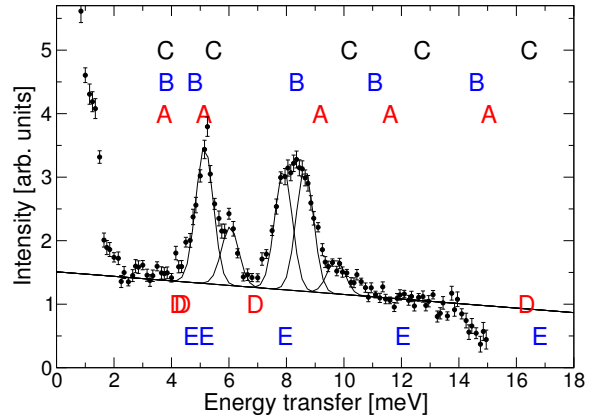
Fig. 3. Magnetic excitations. Points show the INS spectrum obtained on MARI with T = 8 K, E_i = 17 meV and 1 \leq Q \leq 2 \text{ \AA}^{-1} . Lines are Gaussian fits on a linear background. Letters represent numerical results for the S = 9 excitations listed in Table 1 for the corresponding parameter choices. A constant energy 1.29 meV has been added to all calculated energies to account for magnetic anisotropy effects [6].
